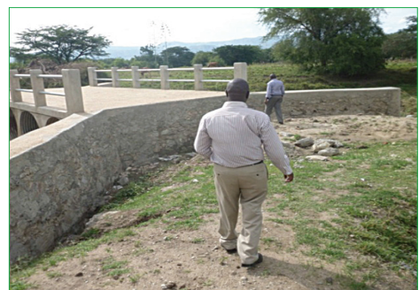
Kakatorogo Bridge Works along Rwebisengo Kiranga road, Ntoroko District nearing completion.
